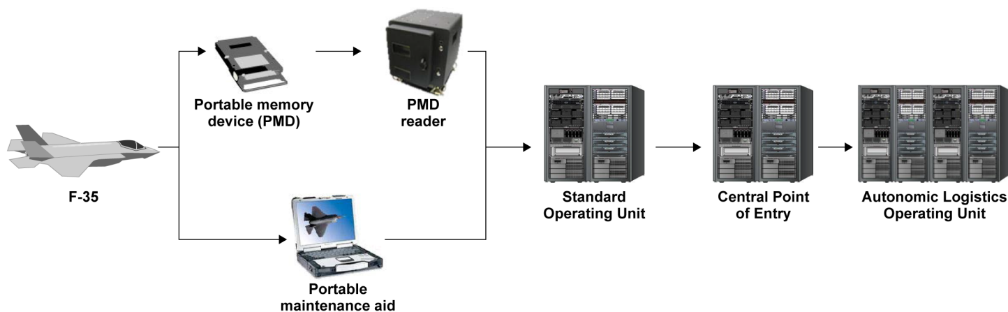
Figure 5: Flow of Unclassified Data from an F-35 Aircraft to the Central Autonomic Logistics Operating Unit
