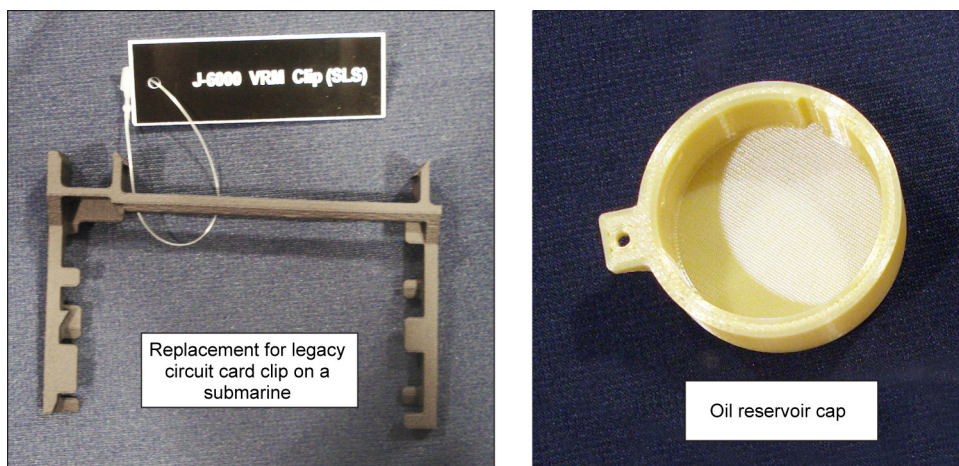
Figure 9: Simple Additively Manufactured Replacement Parts
