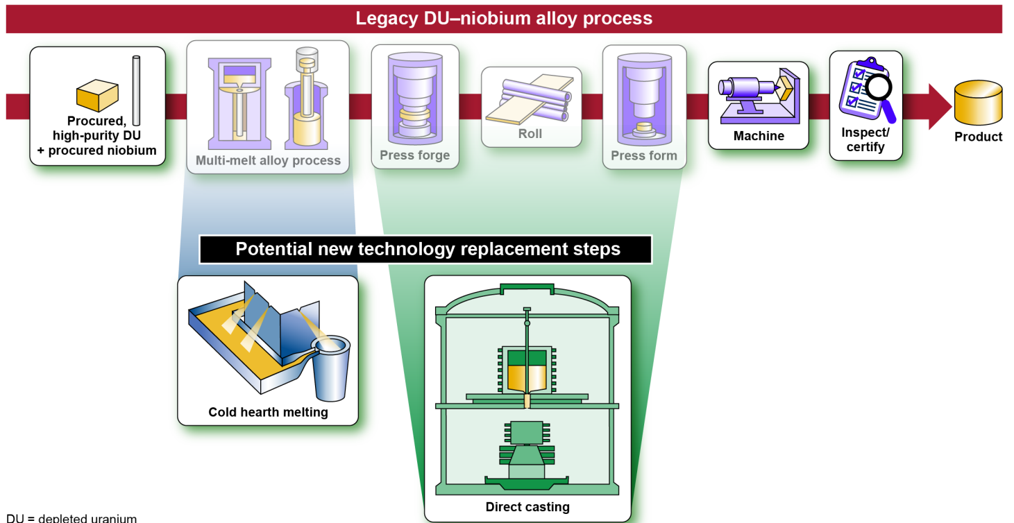
Figure 6: New Manufacturing Technologies for the Depleted Uranium–Niobium Alloy Process
