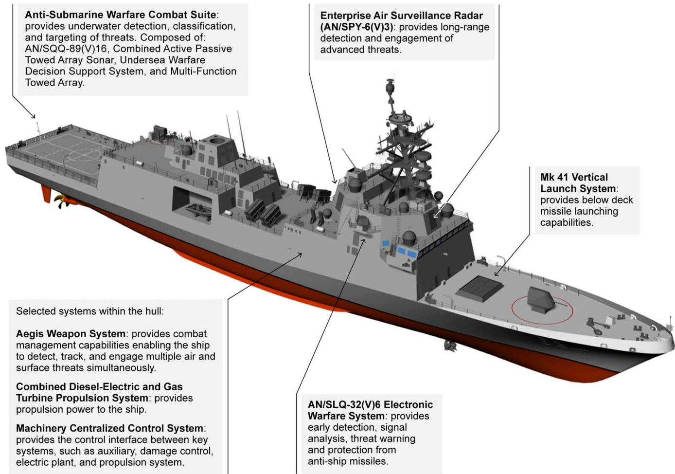
Figure 1: Selected FFG 62 Mission Systems
