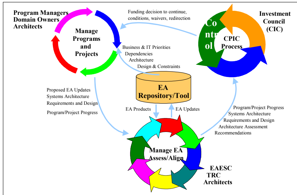
Figure 17. Execute Programs/Projects
